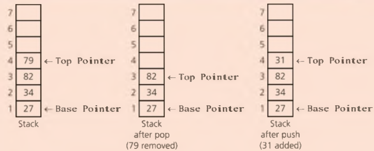
▲ Figure 7.21 Stack operations
