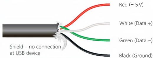
▲ Figure 2.12 Typical USB cable
