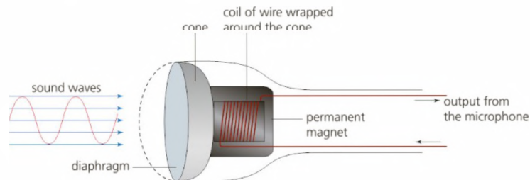
▲ Figure 3.26 Diagram of how a microphone works
