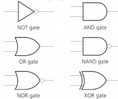
▲ Figure 10.1 Logic gate symbols
