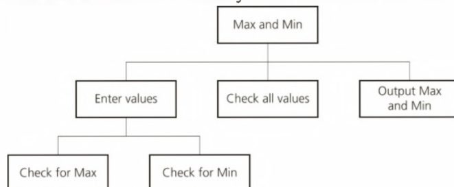
▲ Figure 7.18 Structure chart for Max and Min
