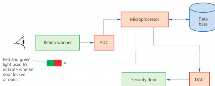
▲ Figure 5.16 Security system controlled by retina scanners
