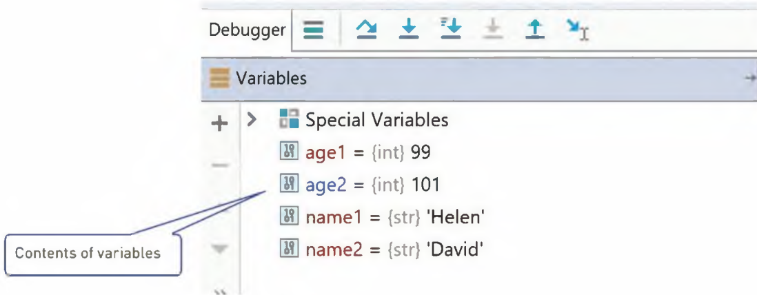
▲ Figure 4.18 PyCharm debugger
