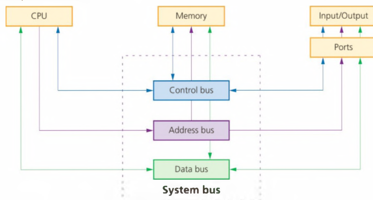
▲ Figure 3.2 System buses and memory
