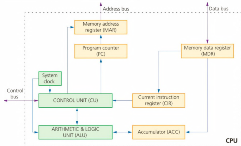
▲ Figure 3.1 Von Neumann architecture
