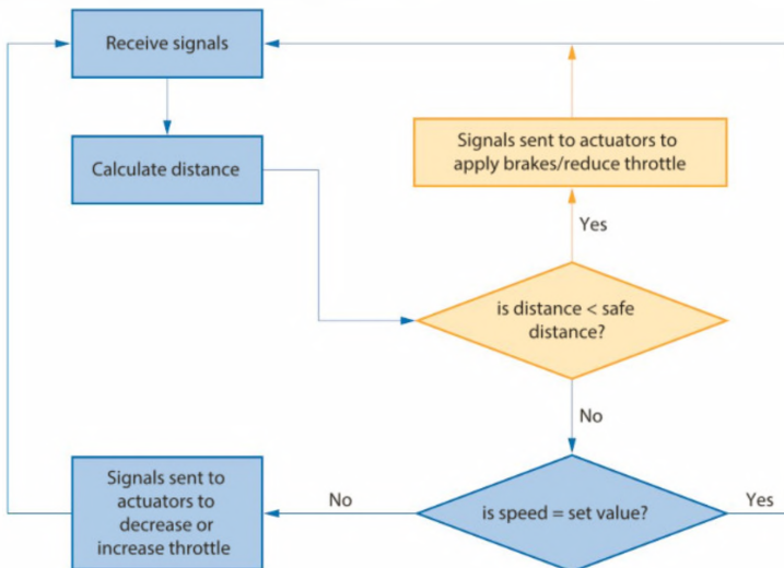
▲ Figure 6.7 Flowchart showing how adaptive cruise control works
