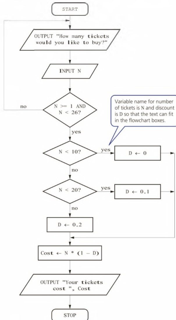
▲ Figure 7.10 Flowchart for ticket cost calculator
