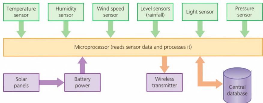
▲ Figure 6.9 Automated weather station
