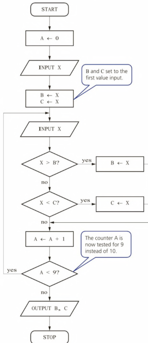
▲ Figure 7.17 A much better algorithm
