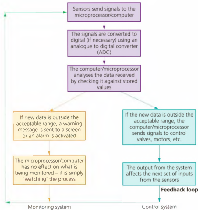
▲ Figure 3.50 Monitoring and control systems using sensors
