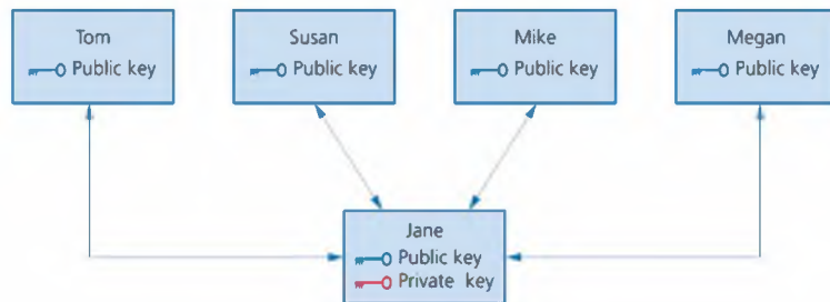
▲ Figure 2.22 The sharing of Jane's public key
