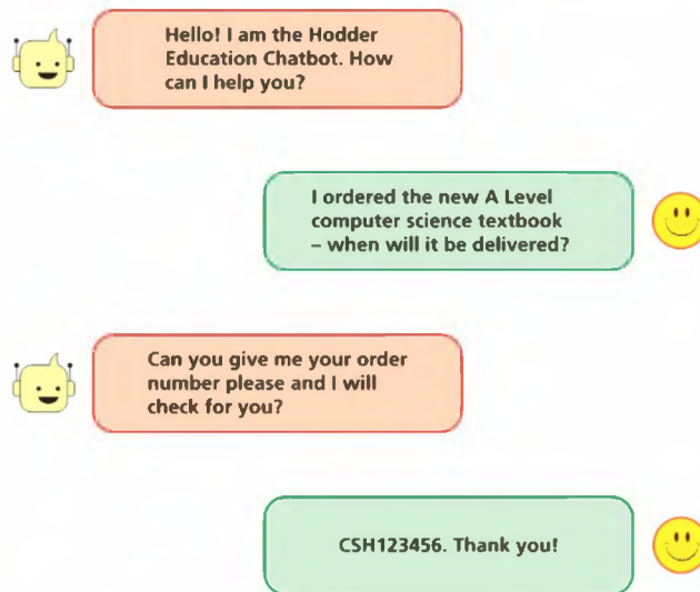
▲ Figure 6.22 Chatbots
