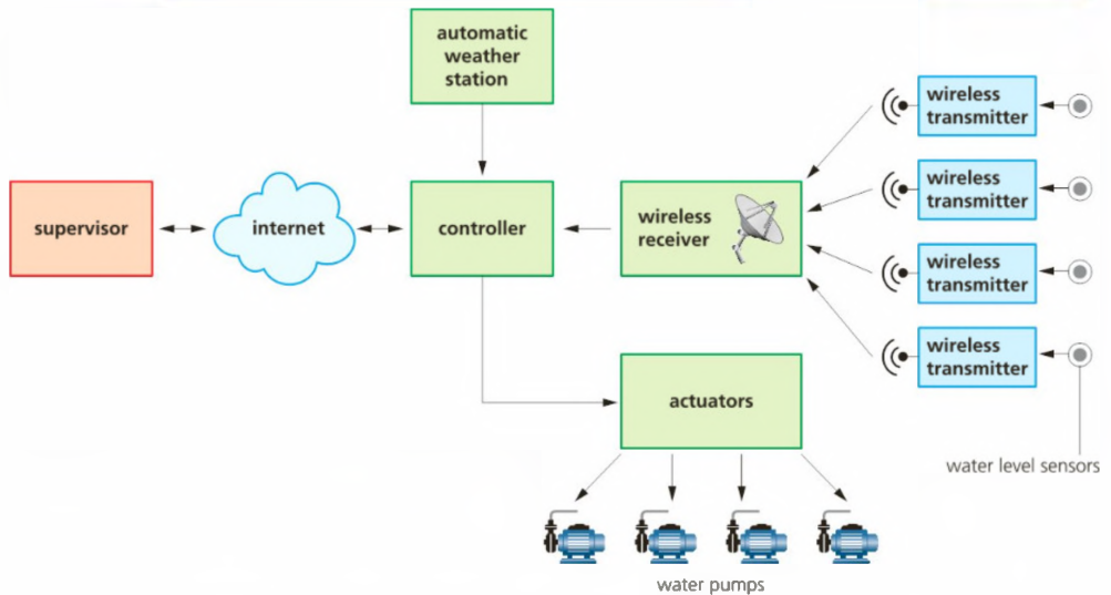
▲ Figure 6.8 Automatic irrigation system
