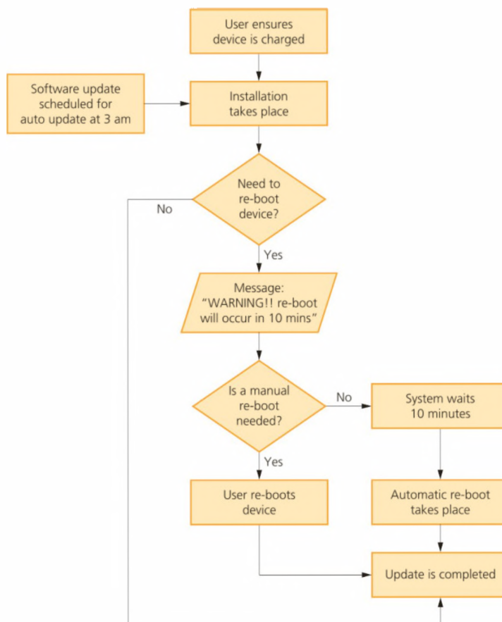
▲ Figure 5.18 Automatic software update flow chart
