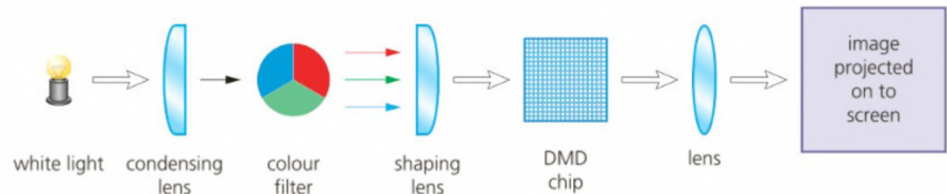
▲ Figure 3.37 A digital light projector [DLP]
