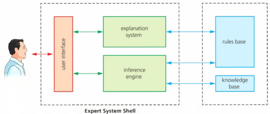
▲ Figure 6.23 Expert system structure
