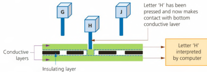
▲ Figure 3.25 Diagram of a keyboard
