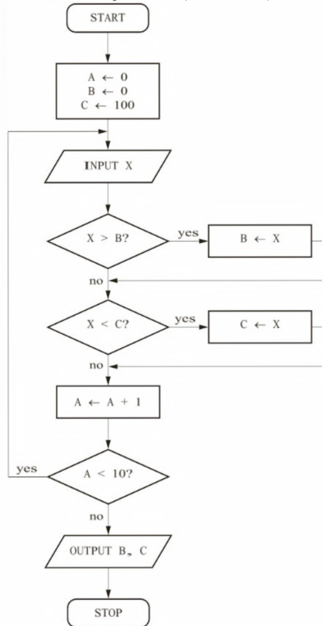
▲ Figure 7.15 Flowchart to trace
