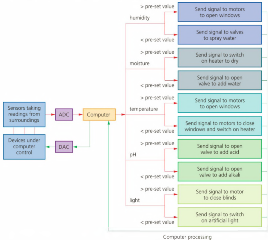
▲ Figure 3.54 Control of greenhouse environment
