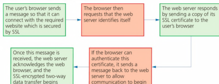
▲ Figure 5.23 Secure sockets layer [SSL]
