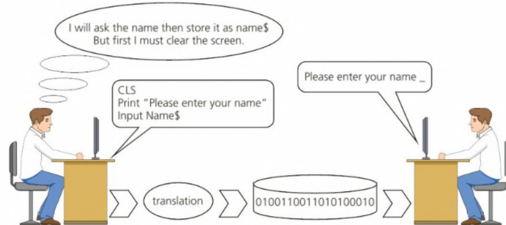
▲ Figure 4.15 Translation
