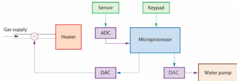
▲ Figure 3.53 Controlling a central heating system
