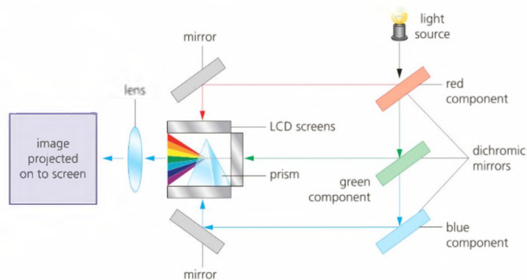
▲ Figure 3.38 LCD projector
