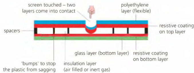
▲ Figure 3.35 Resistive touch screen
