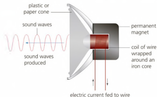
▲ Figure 3.47 Diagram showing how a loudspeaker works
