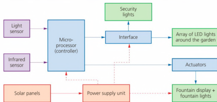
▲ Figure 6.10 Automatic lighting system
