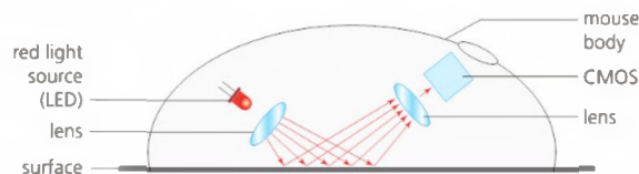
▲ Figure 3.28 Diagram of an optical mouse
