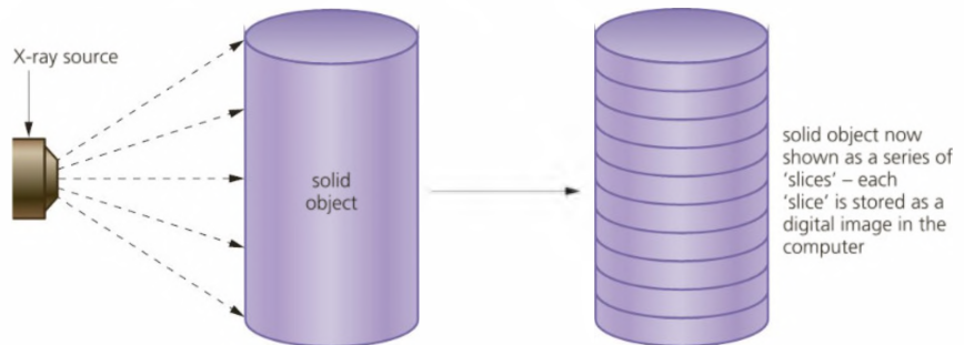
▲ Figure 3.31 Tomography
