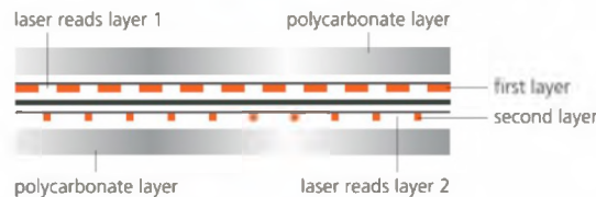
▲ Figure 3.66 Dual-layering on a DVD
