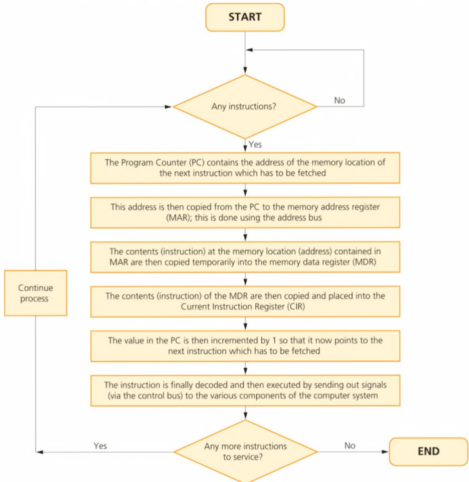
▲ Figure 3.3 Fetch–Decode–Execute cycle flowchart
